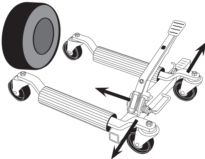
Figure C: Putting Dolly Around Tire (Lever in Down Position)
